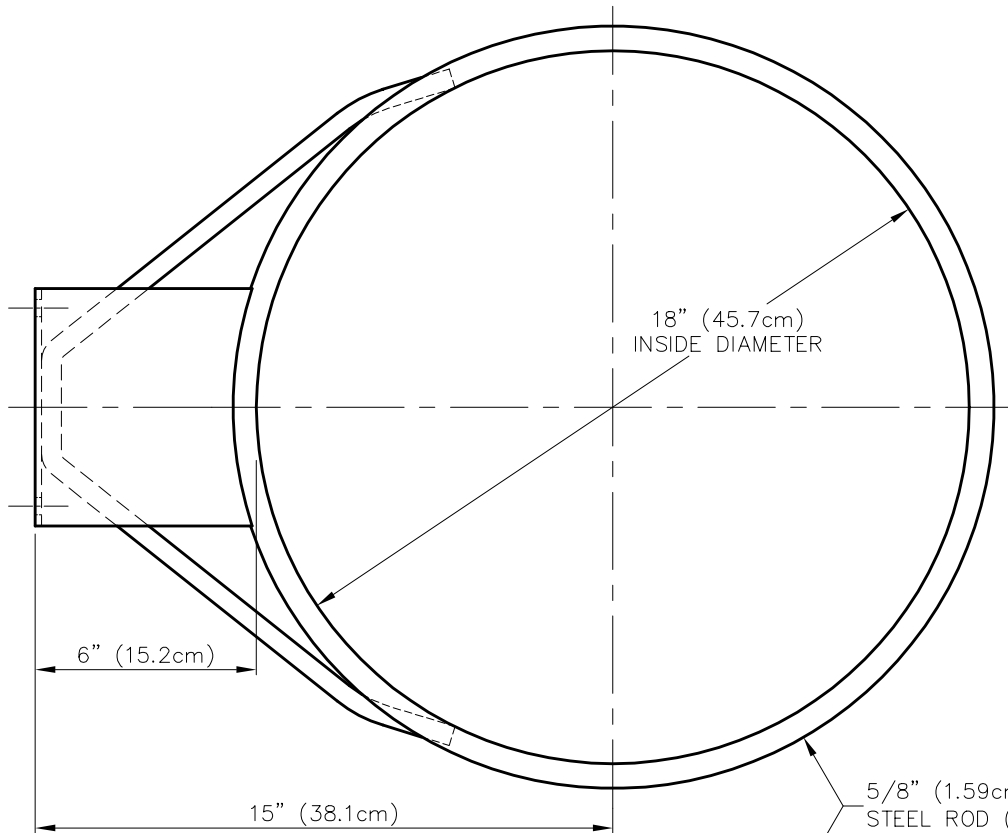
PLAN VIEW
